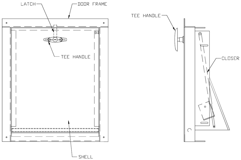
BOTTOM HINGED HAND OPERATED CHUTE INTAKE DOOR
